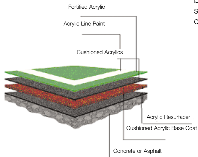
Example cushioned acrylic layering system
